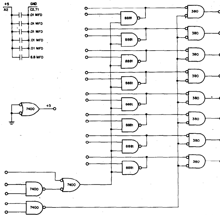
Figure 9.5 M785 Unibus Drivers and Receivers
